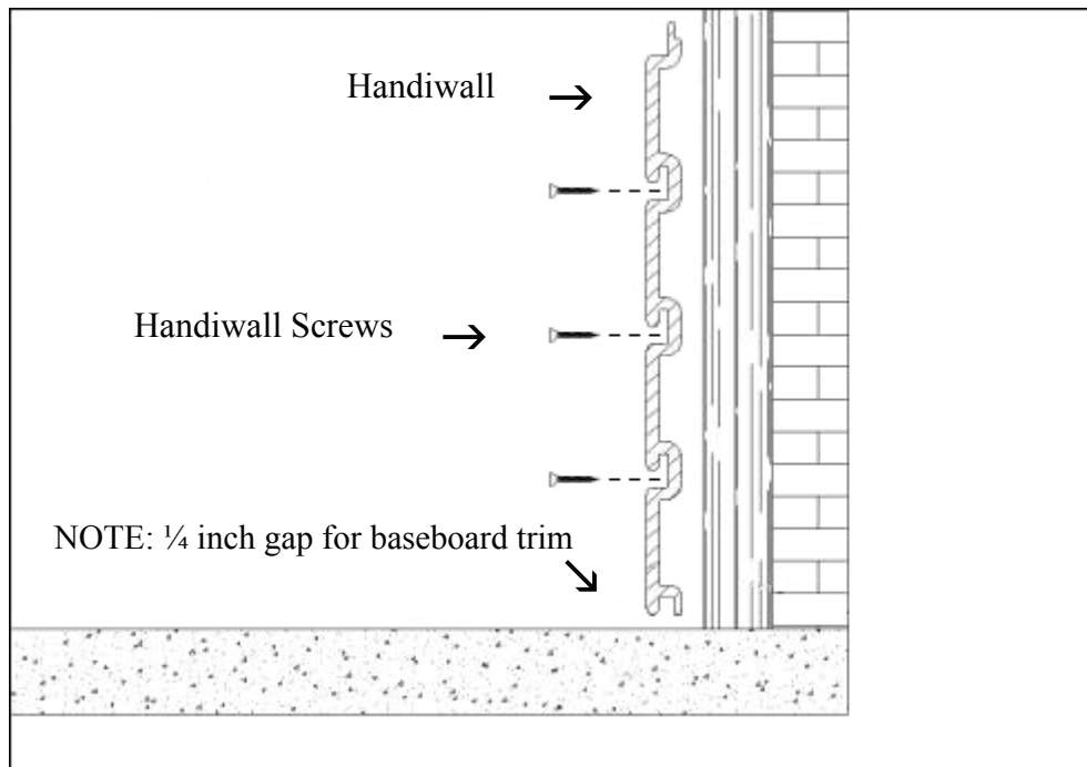
Figure 2. HANDIWALL installation.
